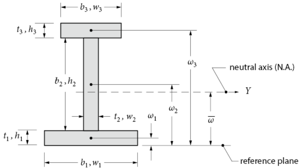
Figure F.3 Geometric properties and location of neutral axis for a general section.
